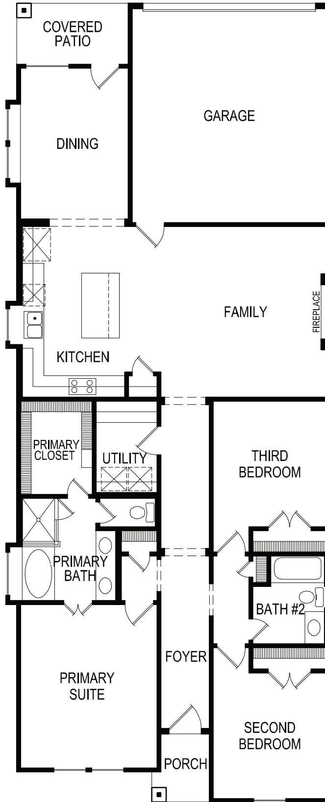
FLOOR PLAN
