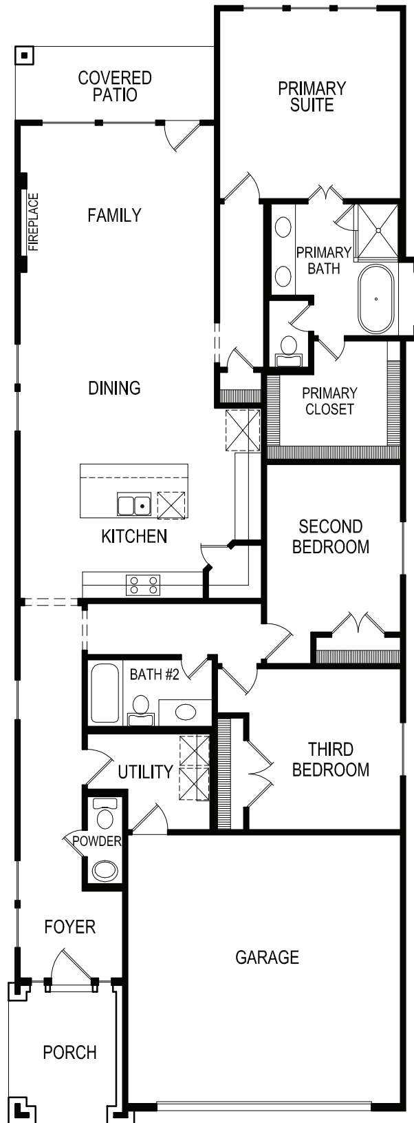
FLOOR PLAN
