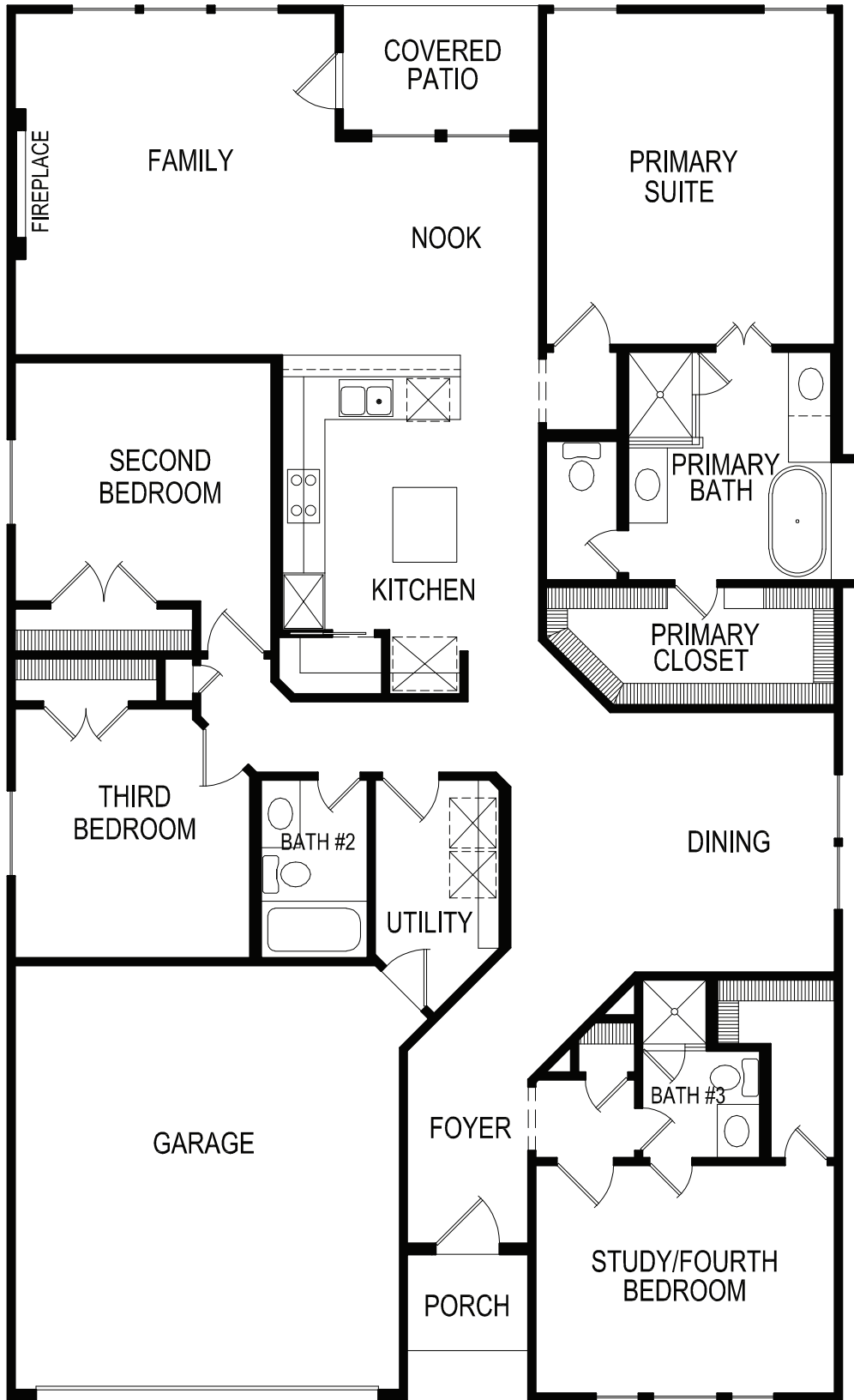
FLOOR PLAN
