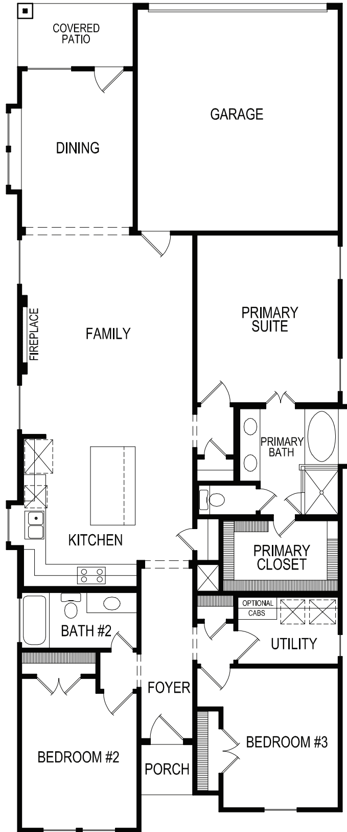
FLOOR PLAN
