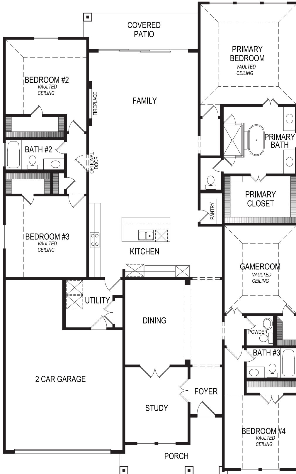
FLOOR PLAN
