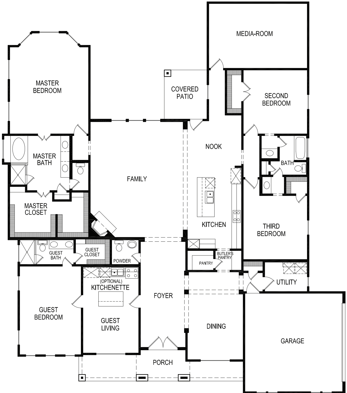
FLOOR PLAN
