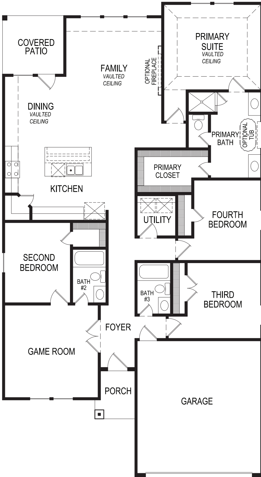
FLOOR PLAN
