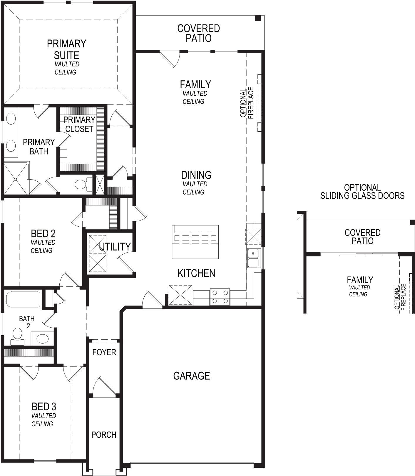
FLOOR PLAN
