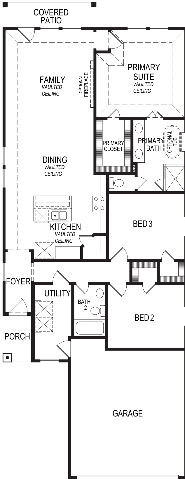
FLOOR PLAN
