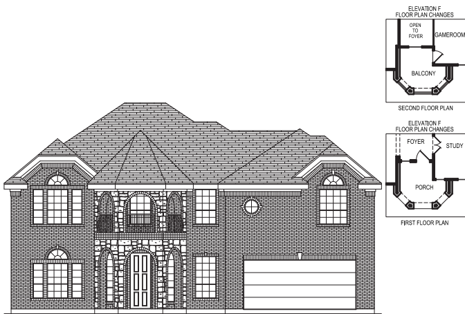
ELEVATION F
