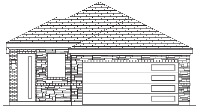
ELEVATION H
