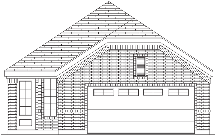
ELEVATION C
